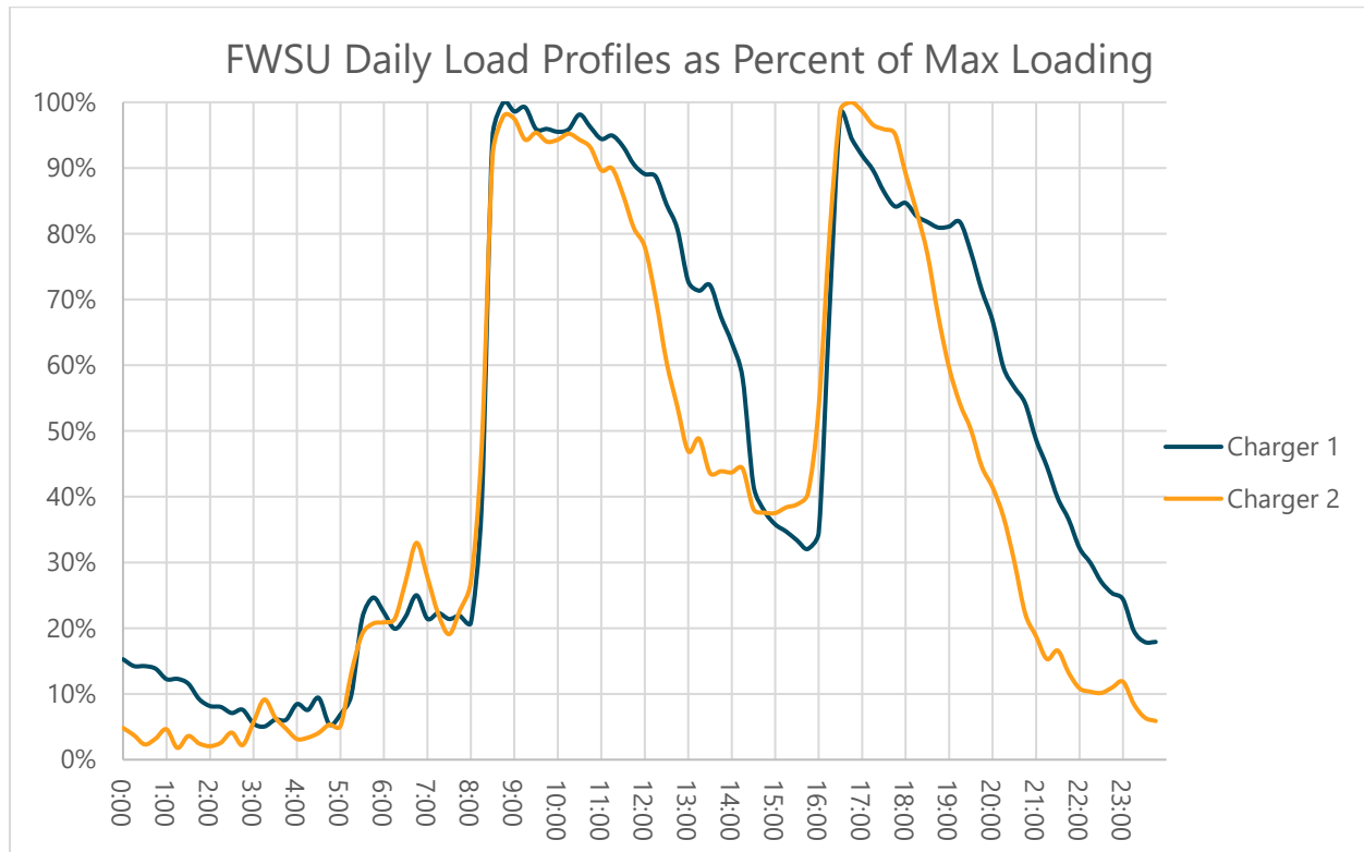
Figure 11: FWSU Daily Load Profiles as Percent of Max Loading
