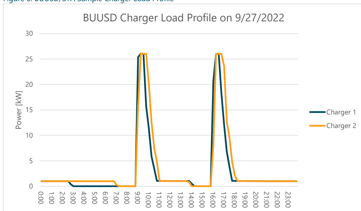
Figure 6: BUUSD/STA Sample Charger Load Profile
